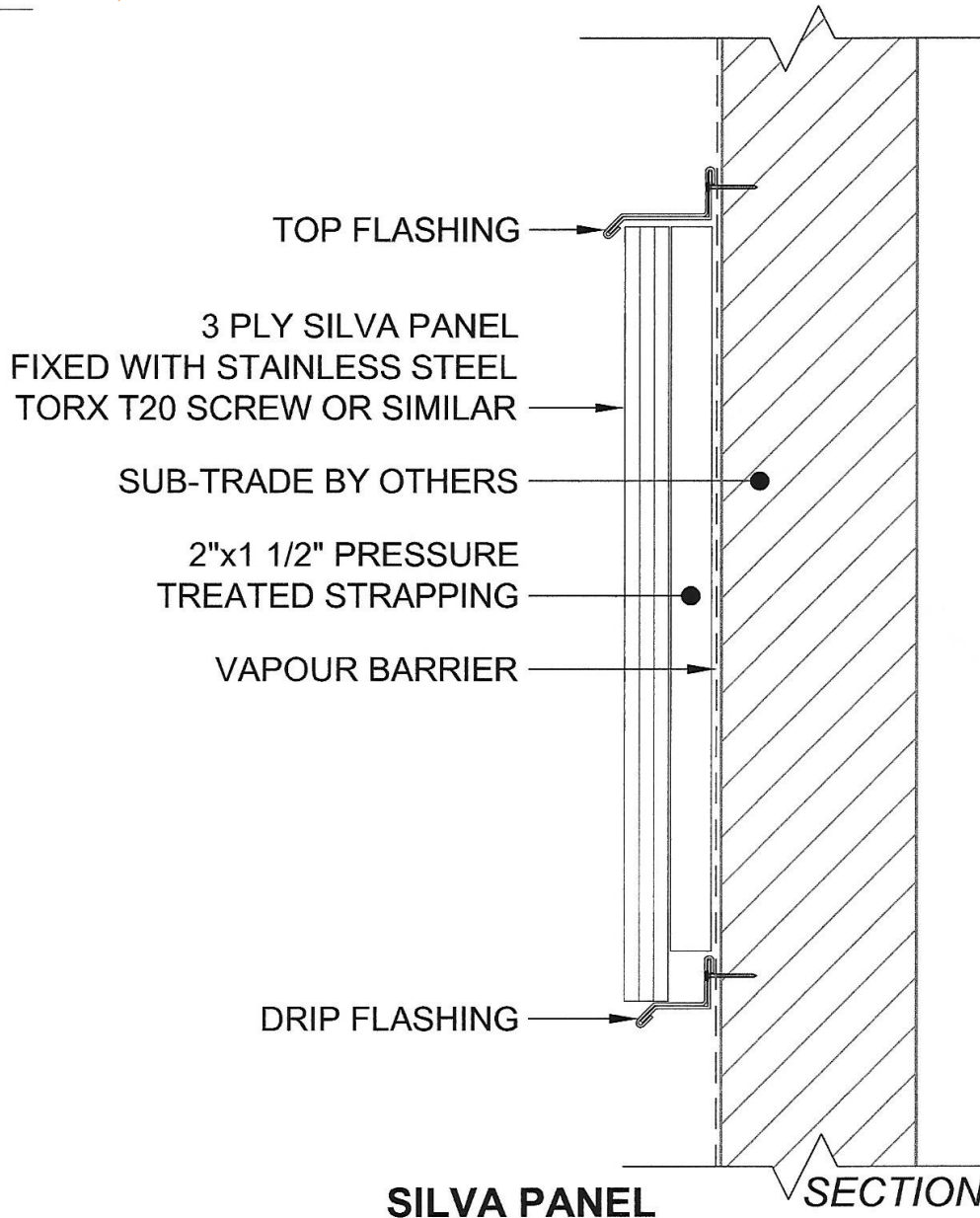
TYPICAL APPLICATION DETAIL ON PRESSURE TREATED STRAPPING
