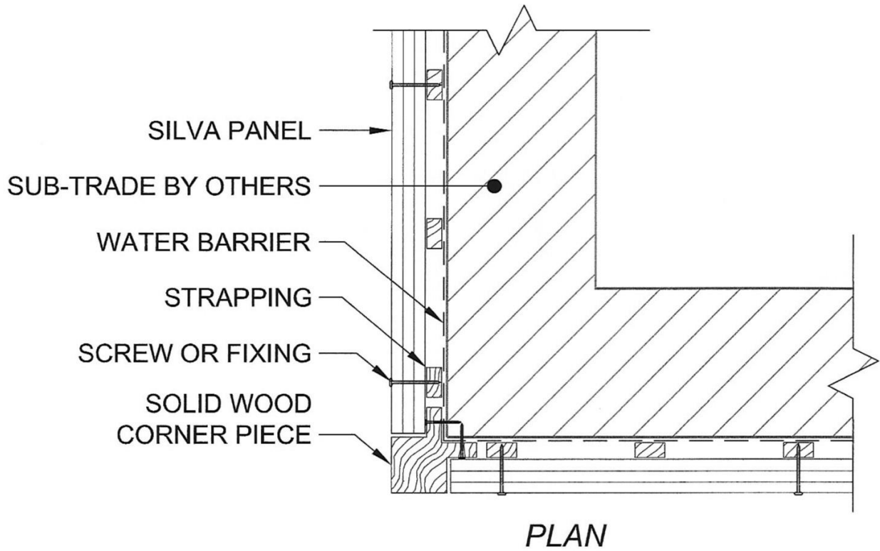
SILVA PANEL TYPICAL CORNER DETAIL
