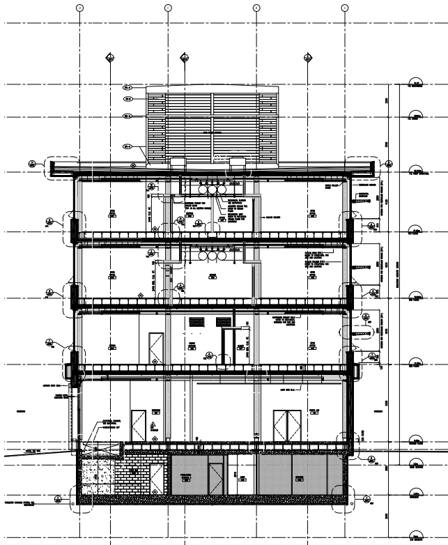
CLT Enclosure Band Option - Section at loading bay looking east Courtesy: Fast + Epp
