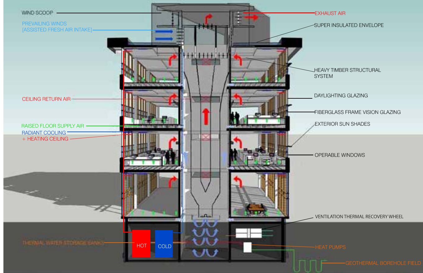
Natural Hybrid Ventilation / Thermal Recovery Systems and Environmental Features Courtesy: Proscenium Architecture
