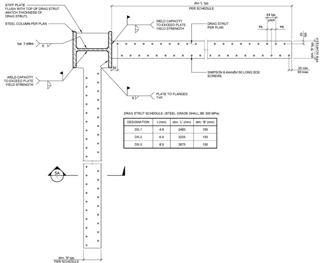
Typical Drag Strut Plan View Courtesy: Fast + Epp
