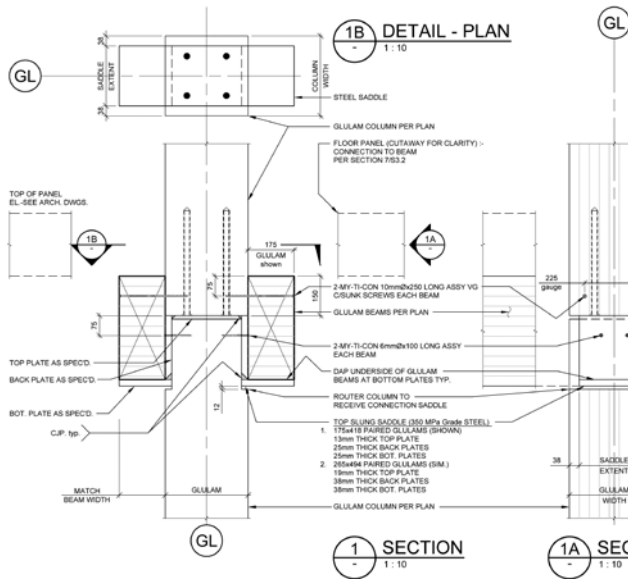
S5.6 Sections and Details Courtesy: Fast + Epp
